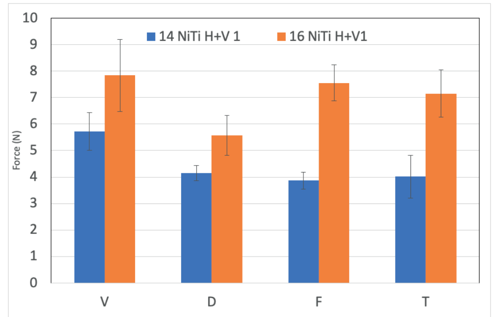
Fig 14: Force generated in tested Groups in Horizontal and Vertical malalignment of 1mm
