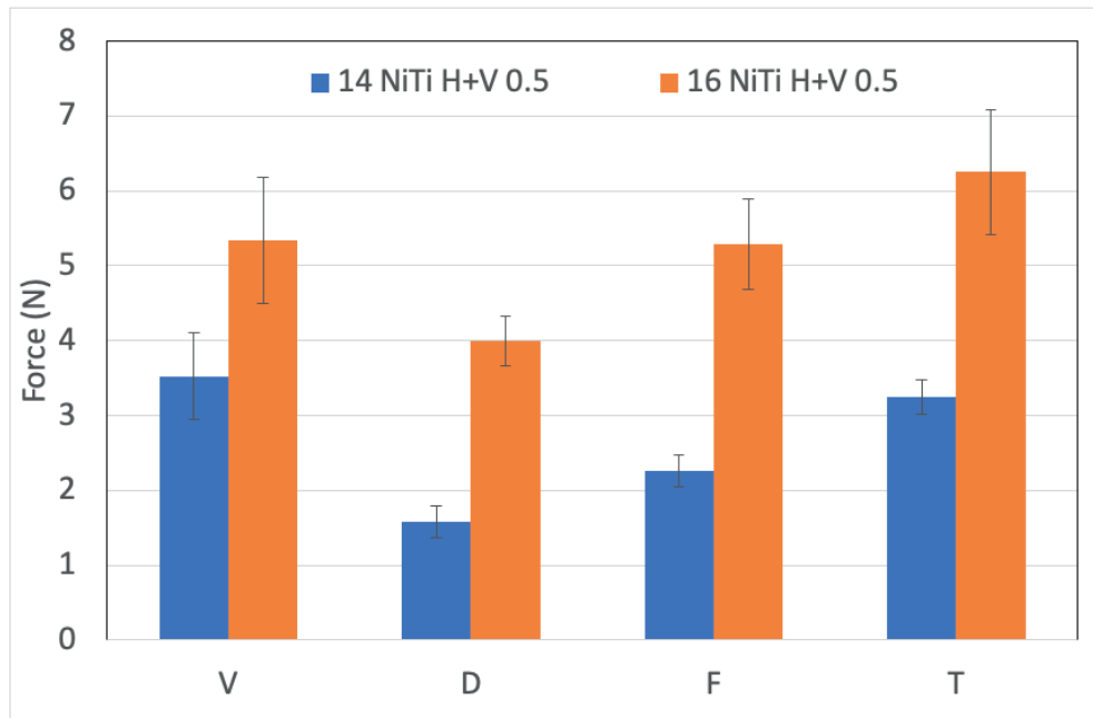
Fig 13: Force generated in tested Groups in Horizontal and Vertical malalignment of 0.5mm
