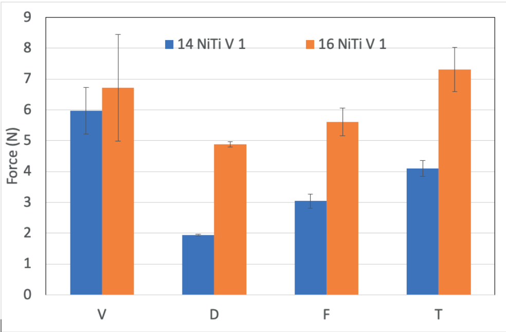
Fig 11: Force generated in tested Groups in Vertical malalignment of 1mm
