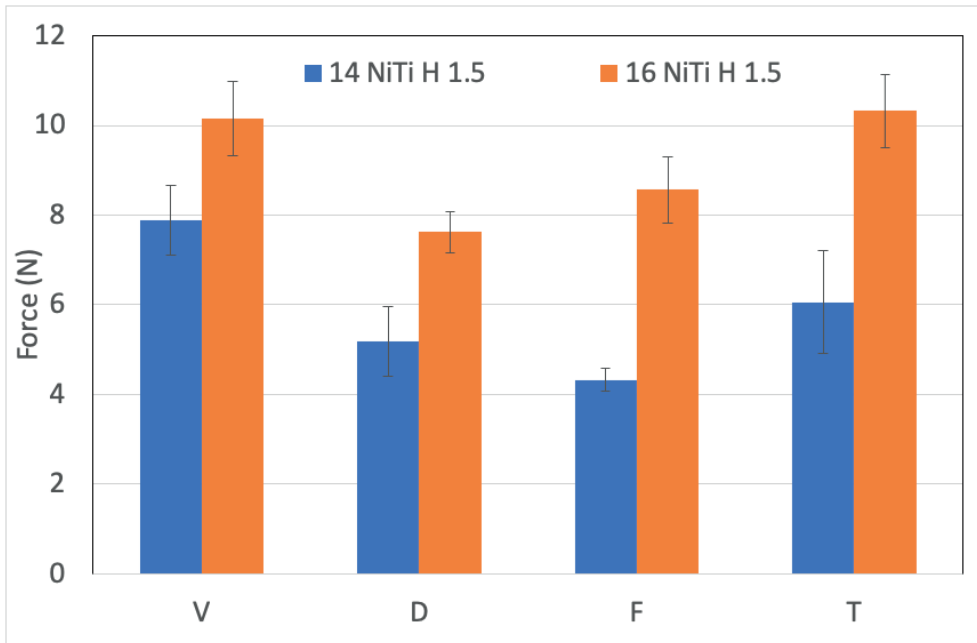
Fig 9: Force generated in tested Groups in Horizontal malalignment of 1.5mm
