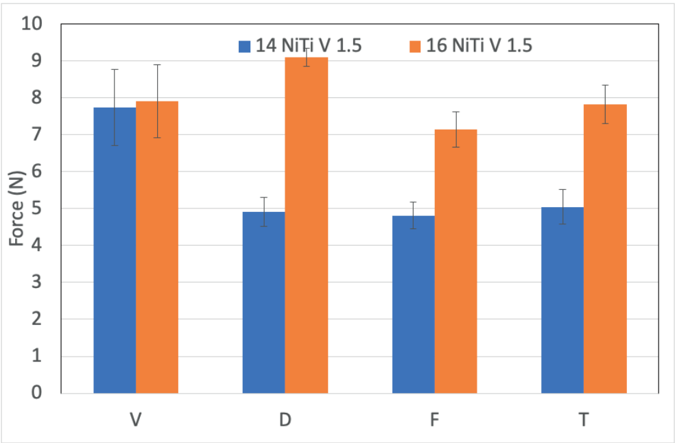
Fig 12: Force generated in tested Groups in Vertical malalignment of 1.5mm
