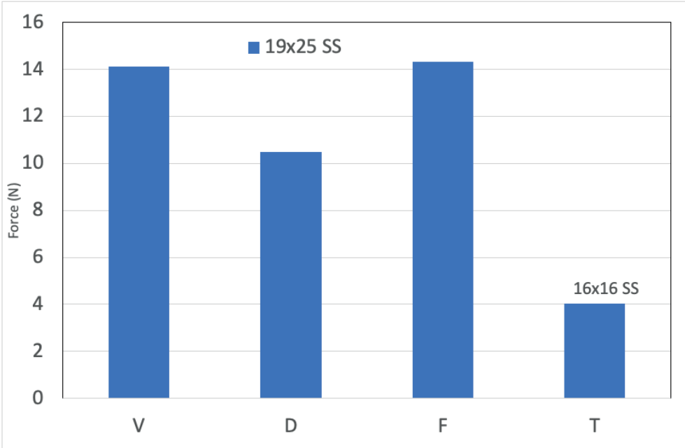
Fig 16: Force generated in tested Groups in no malalignment
