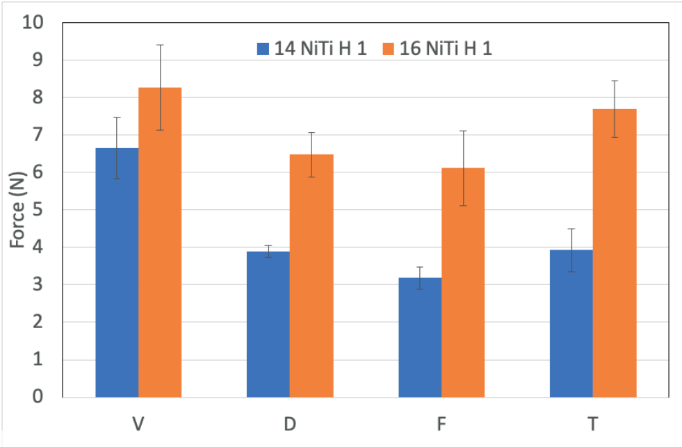
Fig 8: Force generated in tested Groups in Horizontal malalignment of 1mm
